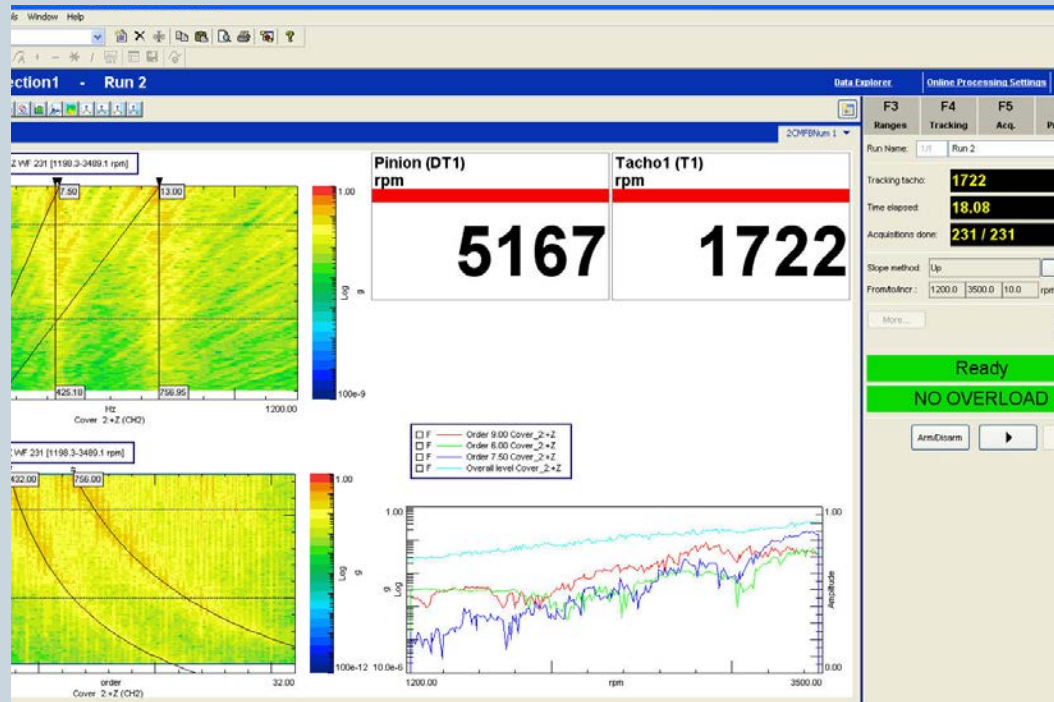
Signature testing with online processing.
