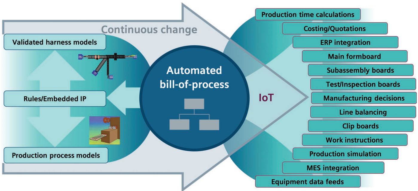
Figure 1. Digital continuity enables a high level of automation in the wiring harness manufacturing process.
