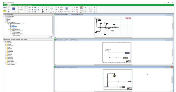
Figure 2. Modern wiring harness engineering solutions help create and maintain effective formboards to improve shop floor processes and efficiency.
