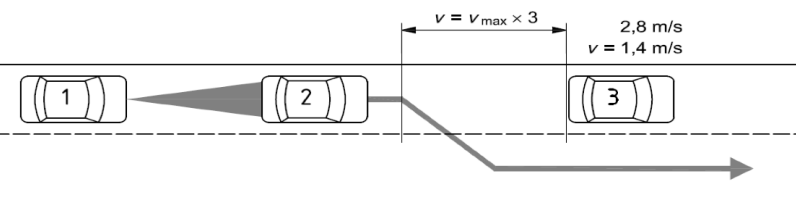
Figure 7: Retargeting test [ISO22178].
