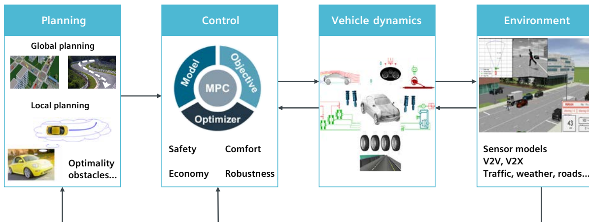
Figure 1: ADAS/AV co-simulation structure.
