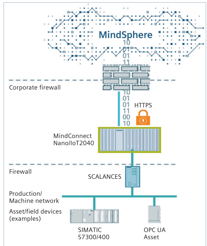
Figure 3: This diagram shows device security, connecting assets to MindSphere.
