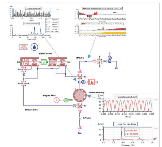
NVH and frequency analysis for a gerotor pump.
