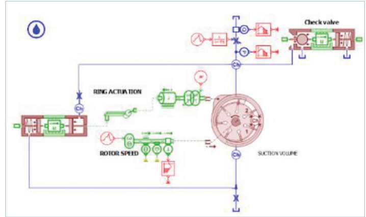
Integrated vane pump submodel.
