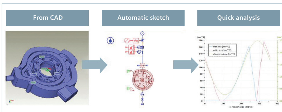
Workflow for an automatic pump sketch generation using CAD import.
