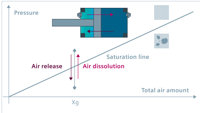
Air dissolution and aeration dynamics.
