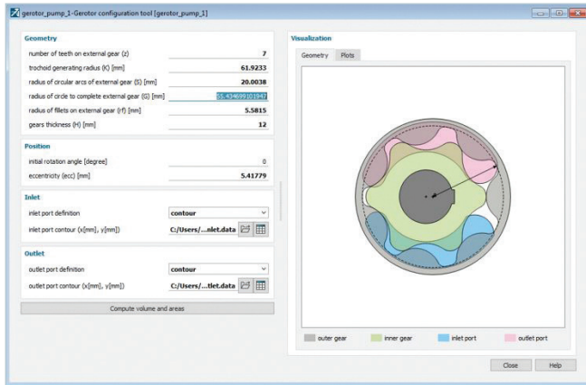
Pump setting tool for gerotor pump.
