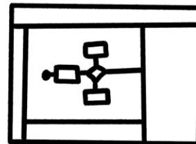
Low-code
