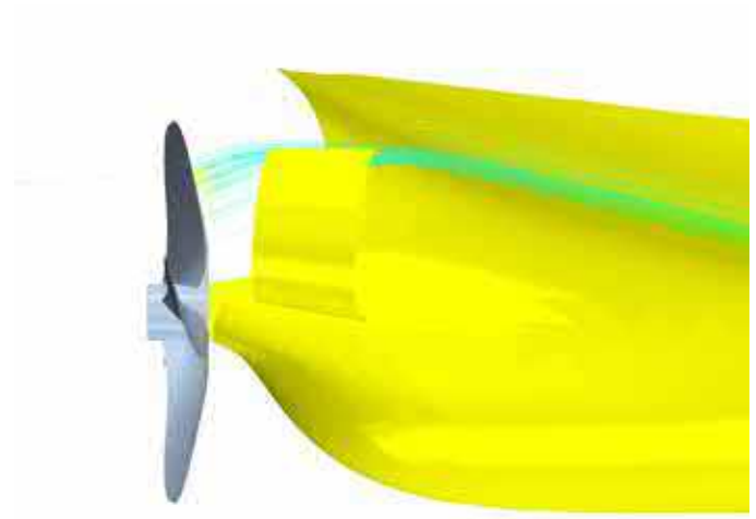
Figure 2: Flow behavior around the duct in ballast draught (6.73 m draught).
