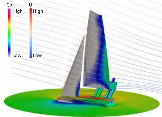
Figure 7: Leeward view of the skiff displaying C_p and streamlines colored to show the flow velocity magnitude, U .
