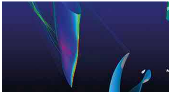
Comparison of the initial and final design of rudder, showing minimal cavitation.
