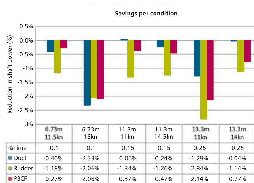
Figure 10: This graph shows the percentage of time allocated to each operating point and the overall savings achieved at each of these points using the three types of ESD.
