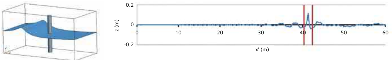
Figure 4: Profile of long crested wave around vertical column.
