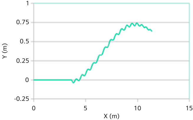
Figure 8: Typical maneuvering trajectory (left) and yaw angle (right).
