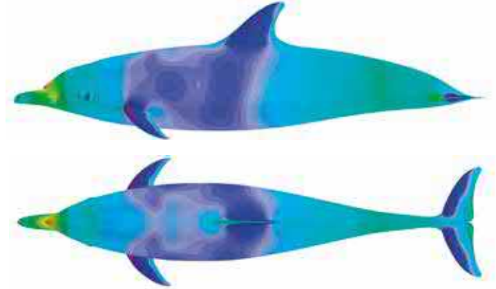
Figure 4: Distribution of pressure coefficient C_p at free-stream turbulence intensity Tu = 1 percent and free-stream velocity u_\infty = 1.0 m/s (side and top views).
