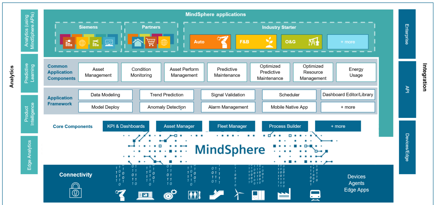
Figure 3: MindSphere architecture.
