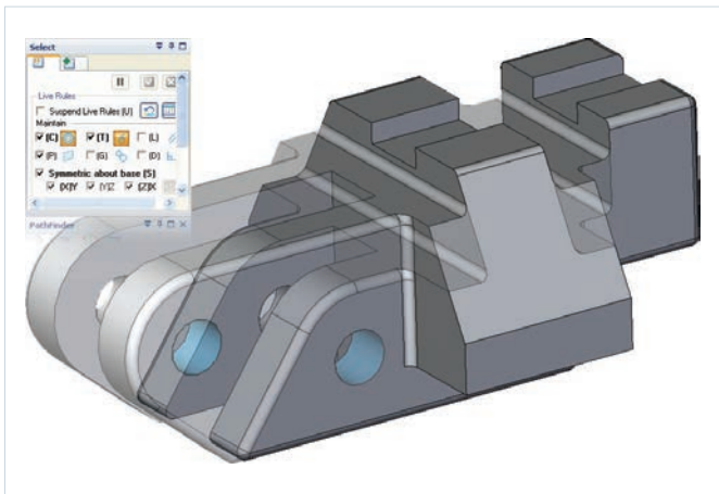
Figure 7: A unique concept in synchronous technology, called Live Rules finds and maintains geometric conditions such as tangent, coplanar and concentric conditions, without explicitly defined constraints. This gives tremendous edit flexibility in making unplanned changes – a similar approach in how 2D is edited.
