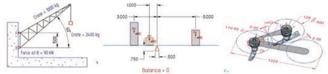
Figure 2: Goal Seek optimizes 2D sketches that simulate a mechanical mechanism, letting designers do "what-if" scenarios before committing to 3D design. As sketches can drive the fit and position of 3D components, Goal Seek provides a simplified way to optimize complex assembly designs.
