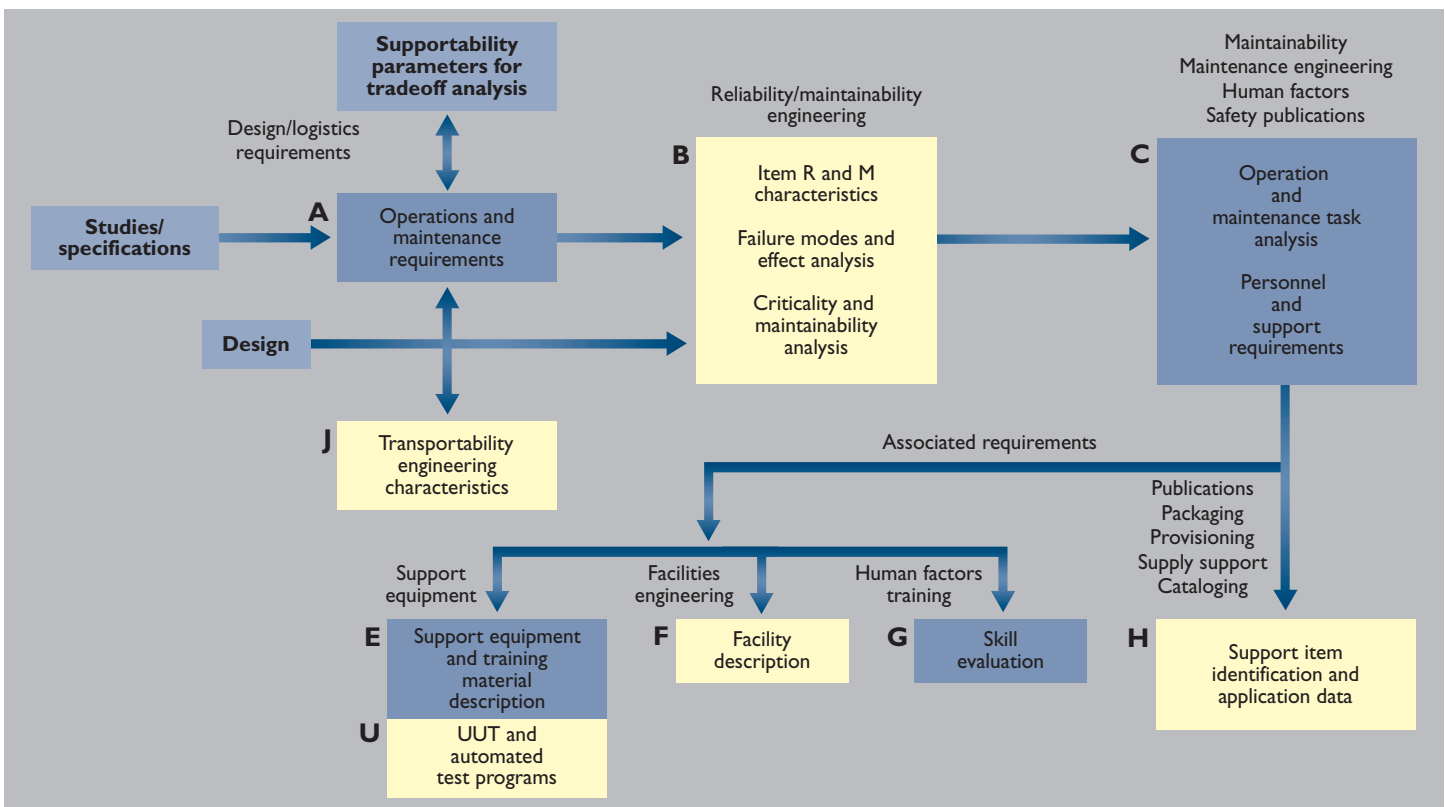
Figure 8: LSAR data flow and system engineering interface
