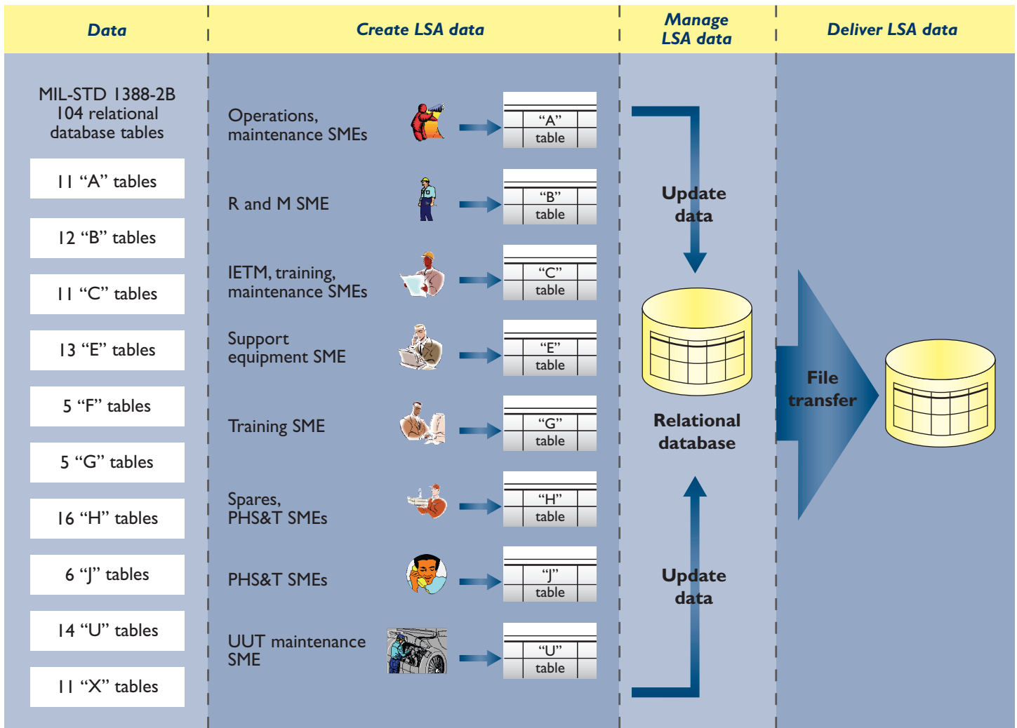
Figure 4: LSA data
