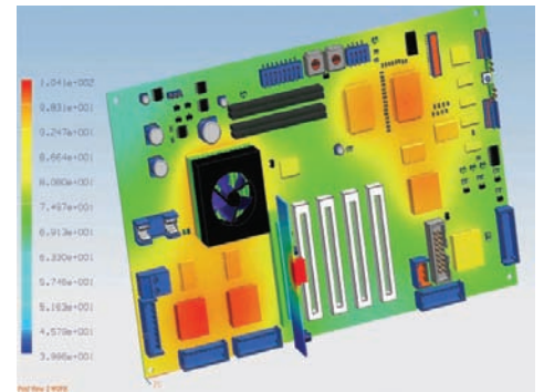
Simulation capabilities include thermal and flow analysis.
